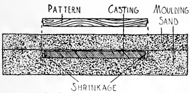
FIG. 515. SHRINKAGE OF METAL IN MOLD.
